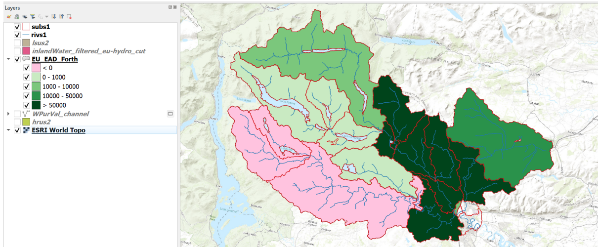
Figure 45. Result of the S+FloodRisk tool for a large-scale peatland restoration simulated in the Forth Basin (UK)
